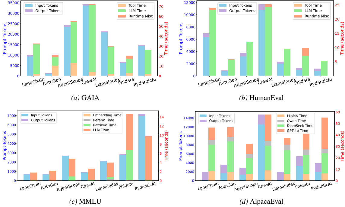
Figure 3. Token consumption and execution time per query of different frameworks.
