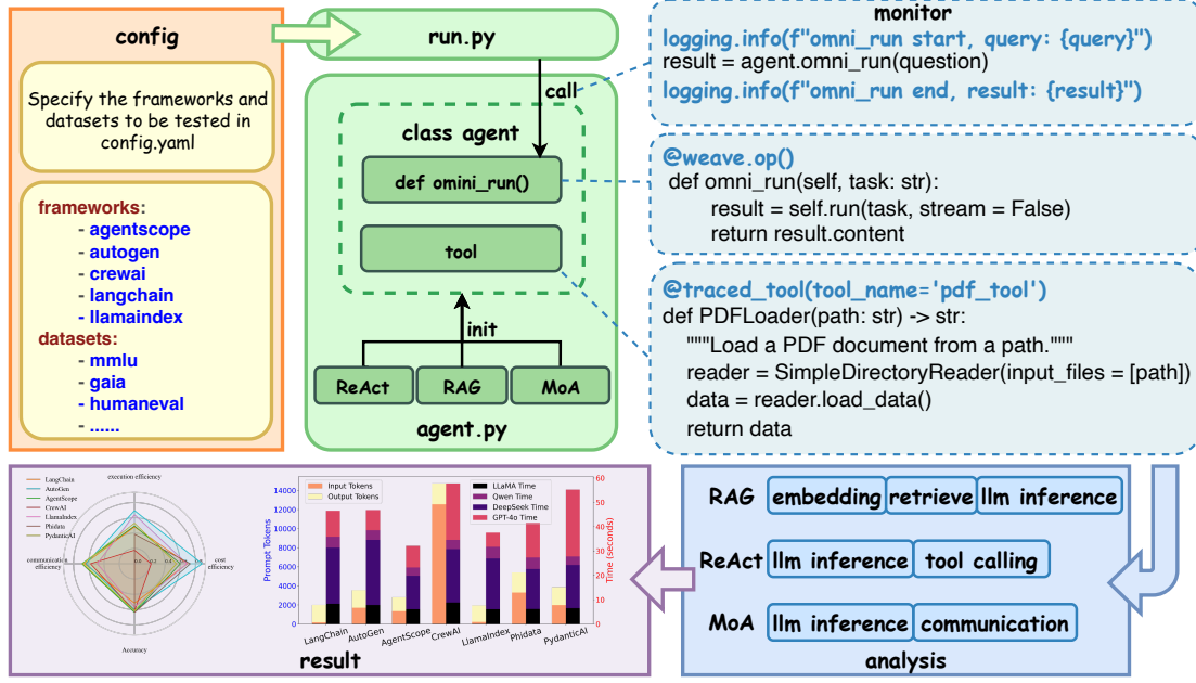
Figure 2. The pipeline of AgentRace.
