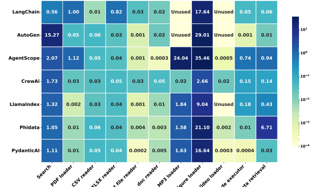
Figure 4. The execution time per call for each tool
