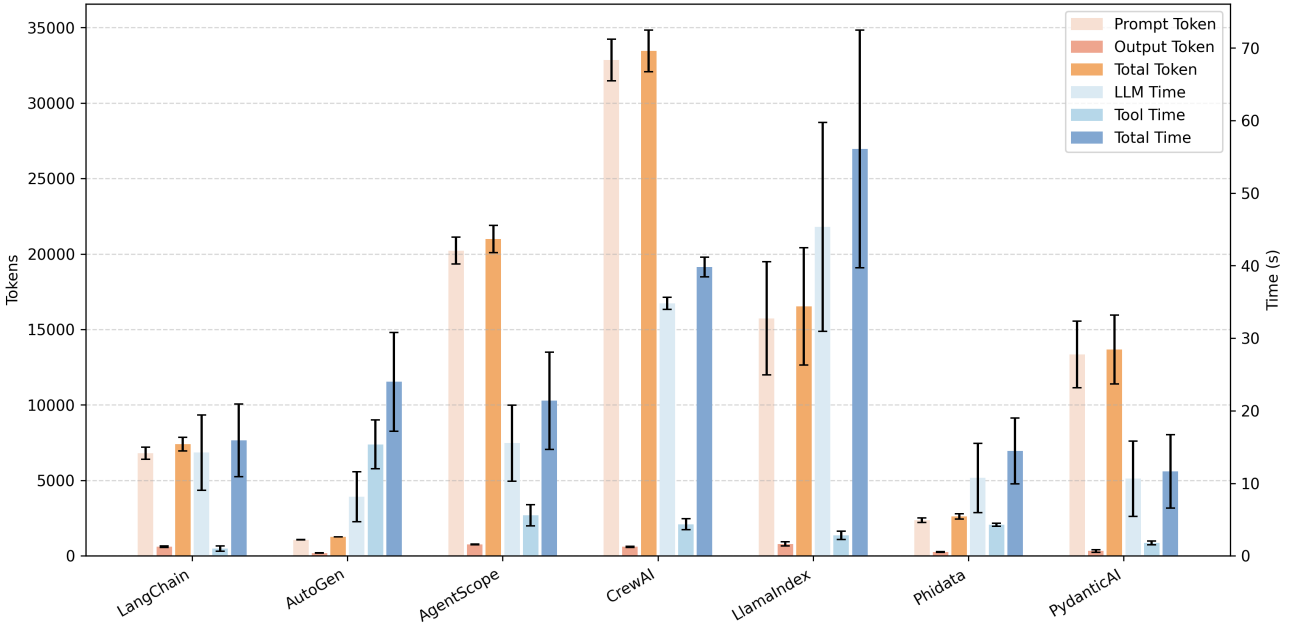
Figure 13. Consistency of Token Consumption and Latency in Repeated Experiments (GAIA)
