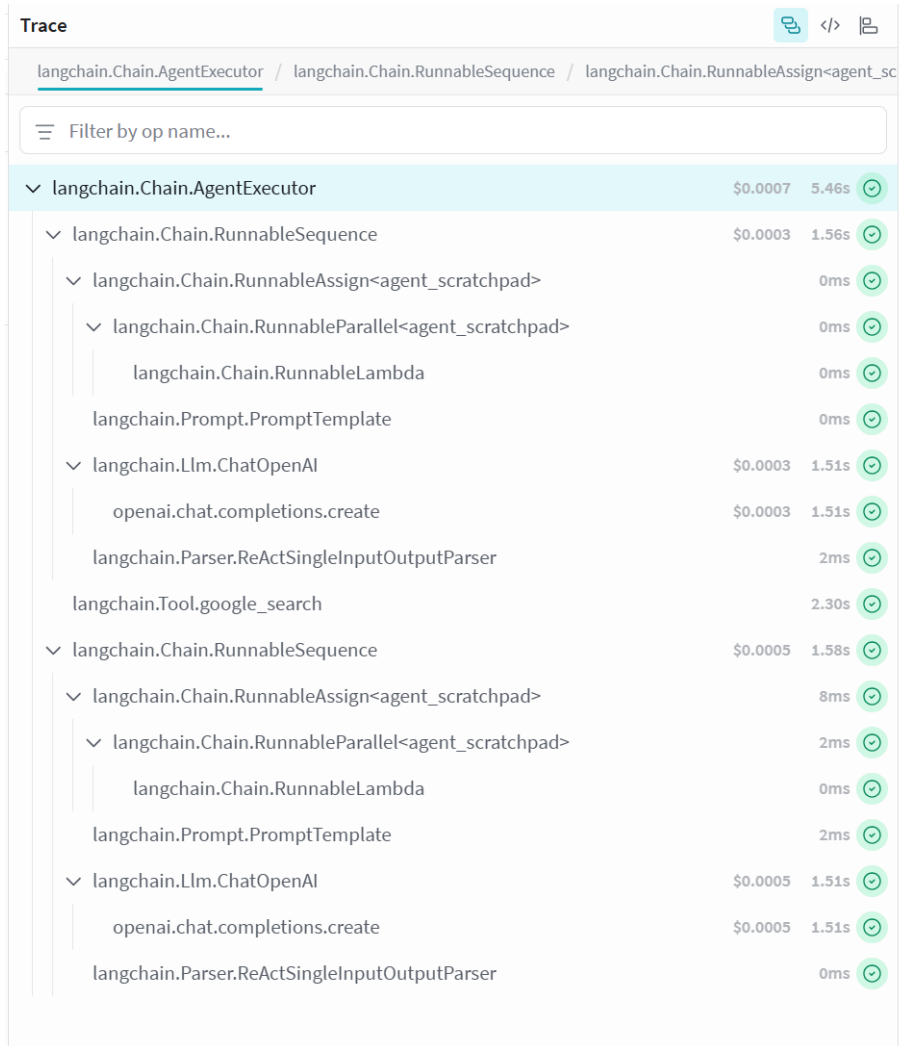
Figure 14. LangChain’s high level of abstraction and encapsulation.
