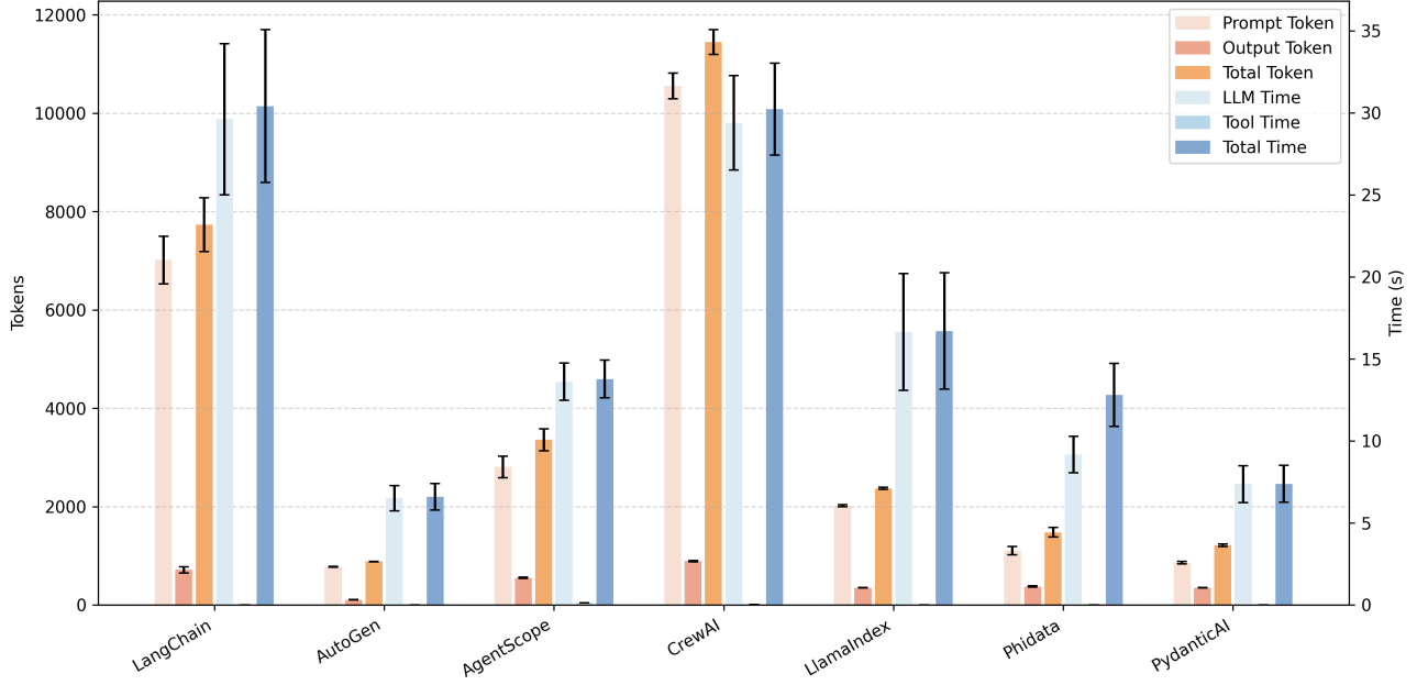
Figure 12. Consistency of Token Consumption and Latency in Repeated Experiments (HumanEval)
