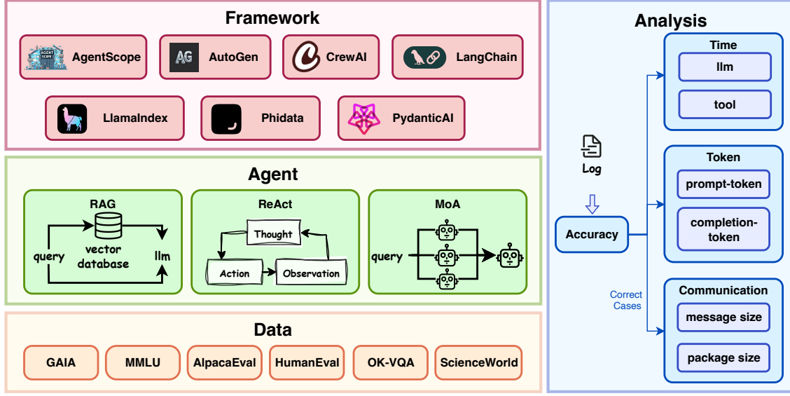
Figure 1. The architecture of AgentRace.
